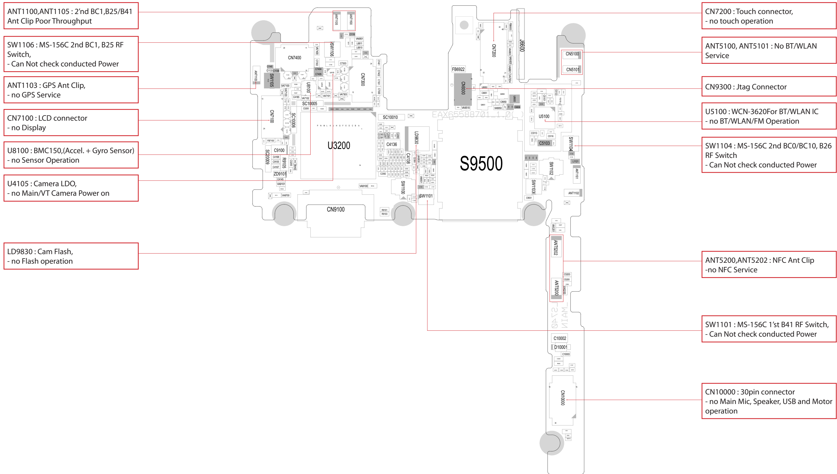
LG-LS740_MAIN_EAX65588701_1.0_BOT-1
